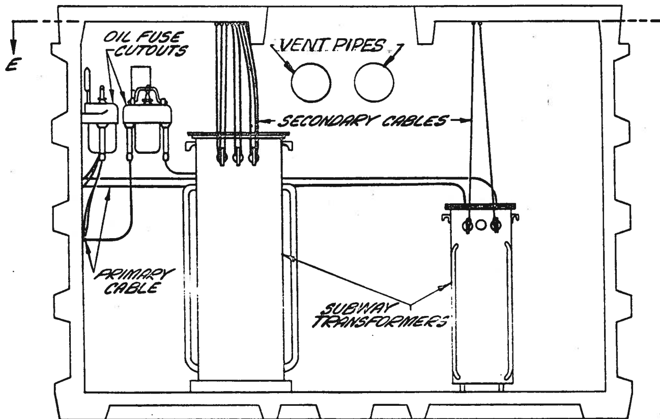
SECTION F-F (FIG. 3)
