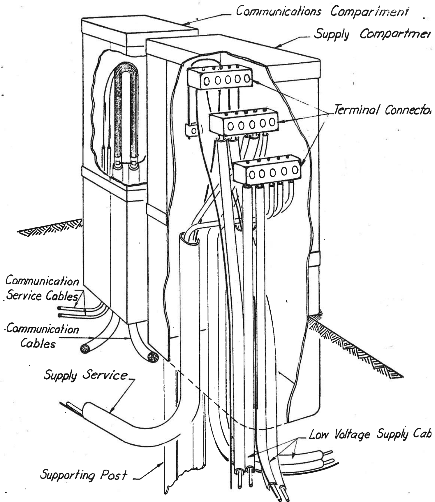
TYPICAL JOINT SUPPLY AND COMMUNICATION PEDESTAL
