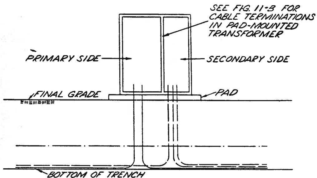
SECTION A - A (FIG. 2)
