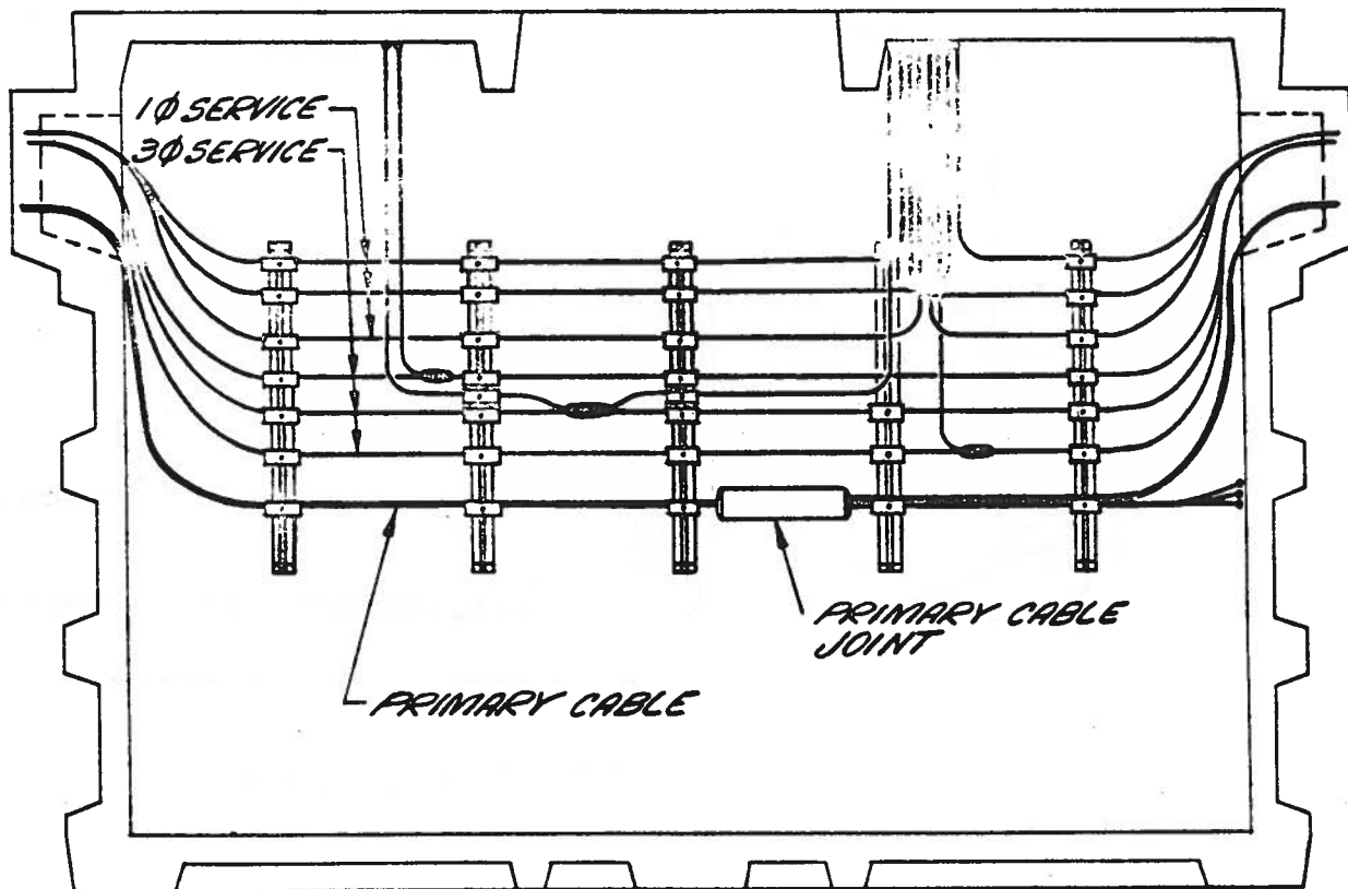
SECTION G-G (FIG. 3)
